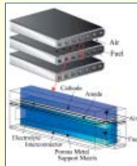
Computational model of the SOFC
